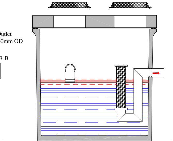
Sec B-B
