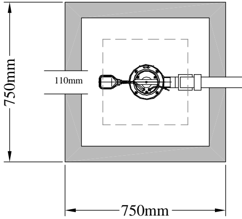
Standard Pumping Station
