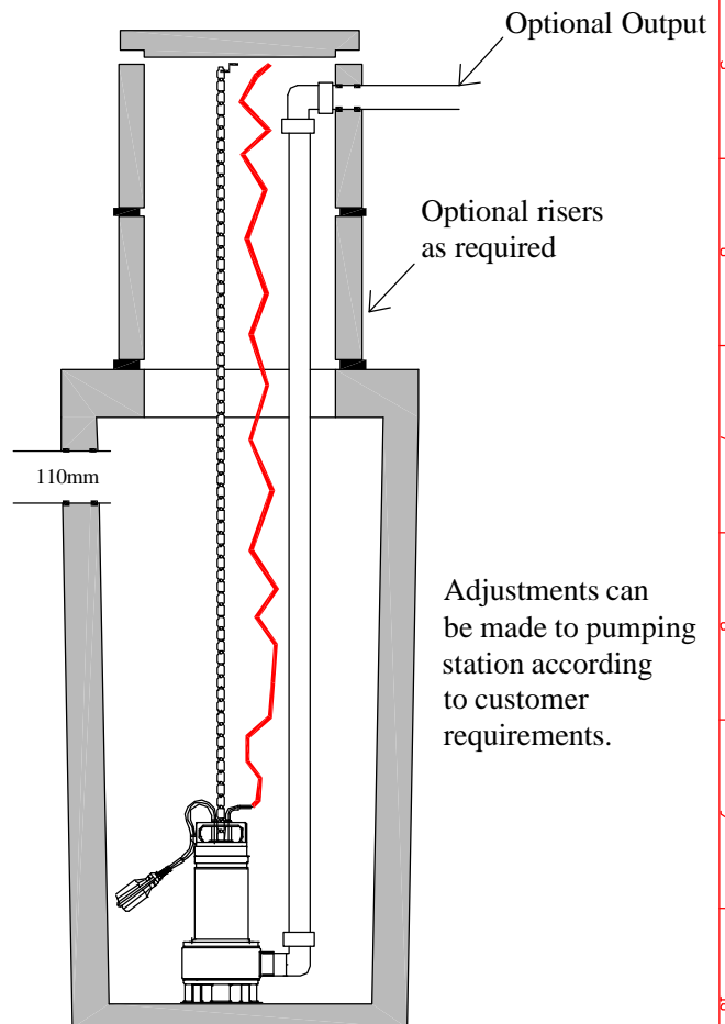
Pumping Station with optional risers
