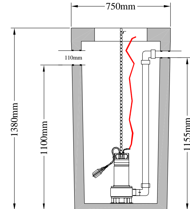
Pumping Station
