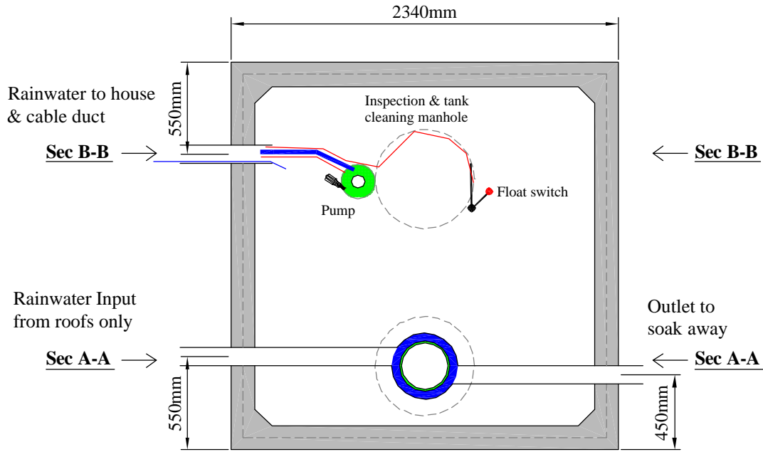
Tank Top Plan
