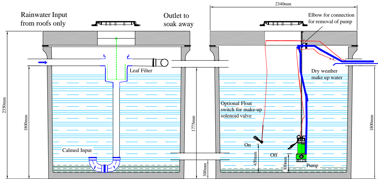
Tanks Vertical Section
