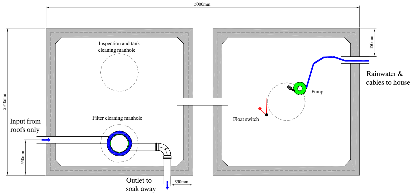
Tanks Top Plan
