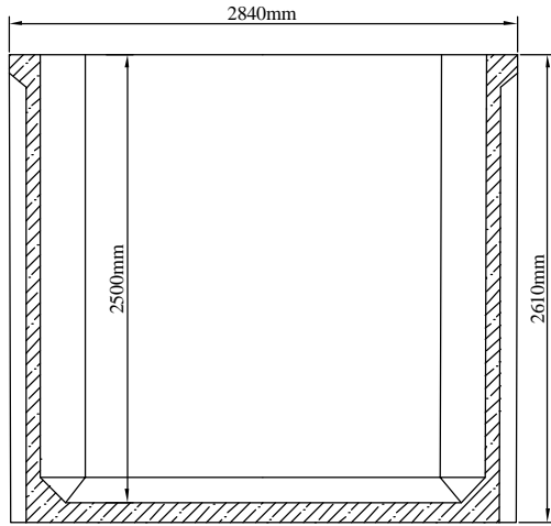
Tank Vertical Section
