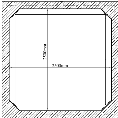
Tank Top Plan
