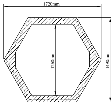
Tank Top Plan
