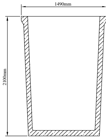
Tank Vertical Section
