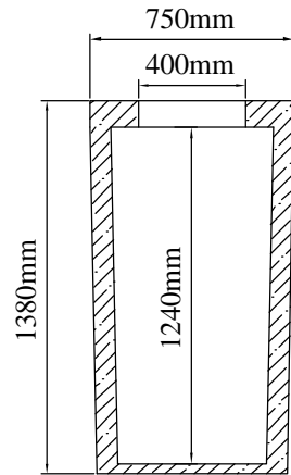
Tank Vertical Section
