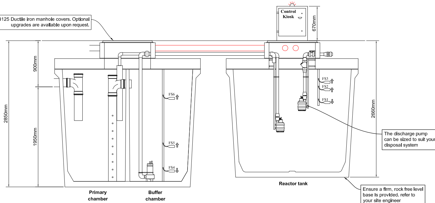
PLAN
