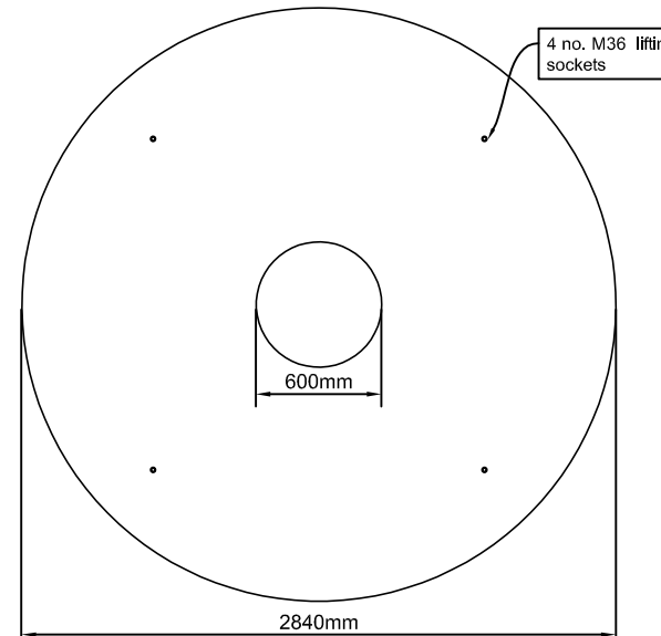
LID PLAN option 2: 600mm opening
