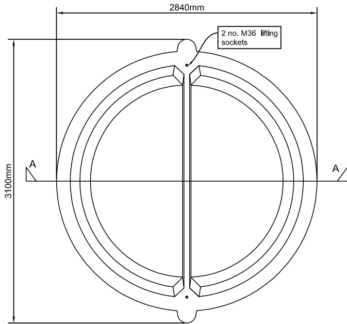
TANK PLAN
