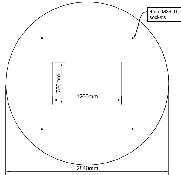
LID PLAN option 1: 1,200 X 750mm opening
