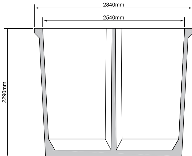
TANK SECTION through A-A
